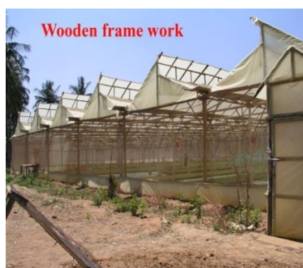
Fig 4: Protected cultivation of Tomato under low cost polyhouse
